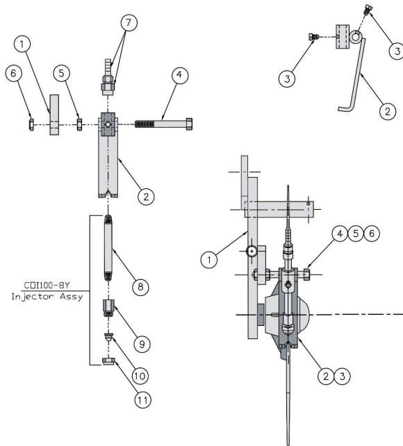
Coulter Injector Assembly
