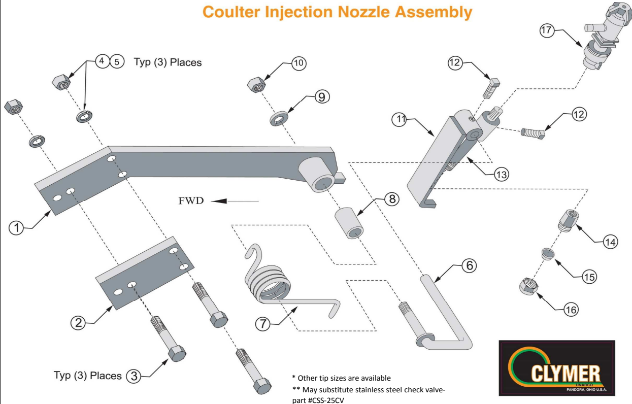
COI100Y - Coulter Injection Bracket and Nozzle Assembly
