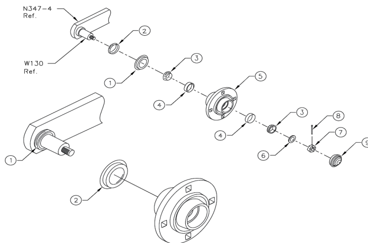
W23Y 4-BOLT HUB ASSEMBLY
